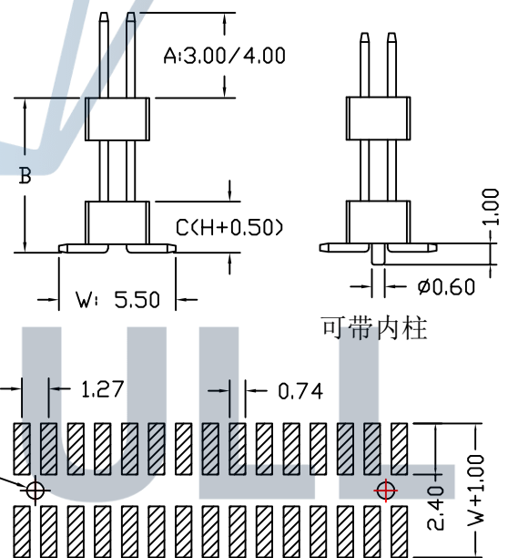
PCB LAYOUT
