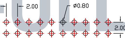
PCB LAYOUT
