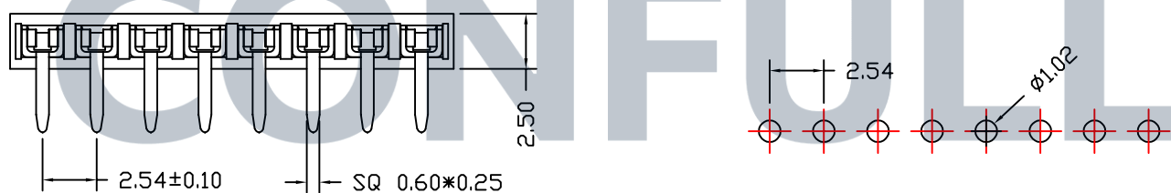
PCB LAYOUT
