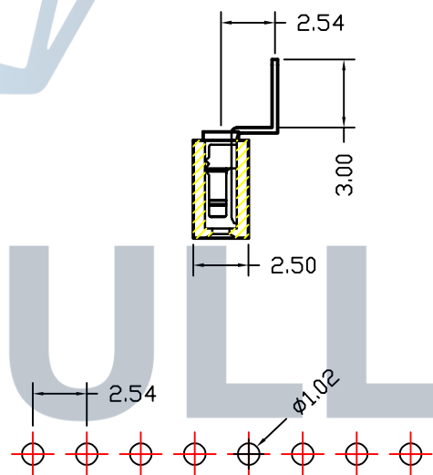
PCB LAYOUT
