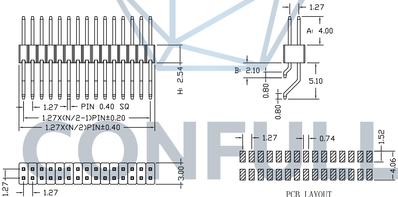
PCB LAYOUT
