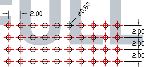
PCB LAYOUT
